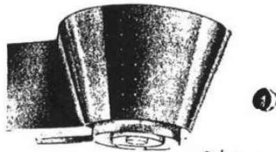
10306: Sculptured perforated brass wall light, free of excessive ornamentation. Soft, even uplight; evenly diffused downlight through concentric brass louver. Depth: 6 1/4"; width: 9"; extension: 12 3/4". Solid Brass. 1-150W.
